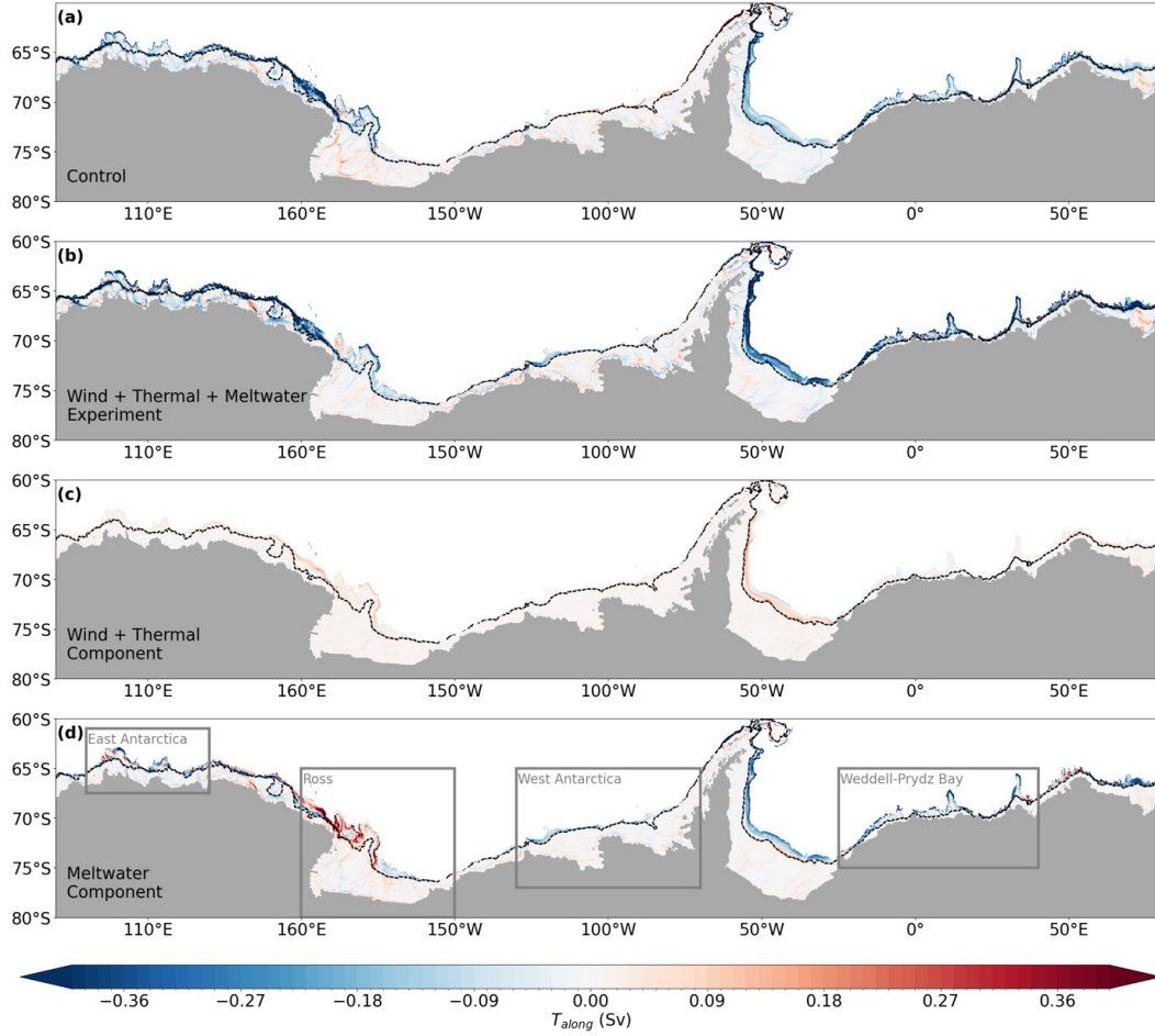
Figure 1. Along-slope depth-averaged transport averaged over 2040-2050 for the (a) Control, (b) experiment with all forcings (Wind+Thermal+Meltwater run) (c) Wind + Thermal component (Wind + Thermal run relative to the control) and the (d) Estimated meltwater component, i.e., (Wind+Thermal+Meltwater run)–(Wind+Thermal run). The dotted line primarily follows the 600m isobath, which we define to separate the ASC and ACoC. The boxes in panel (d) highlight the selected regions featured in Fig. S1 and Fig. S4.
